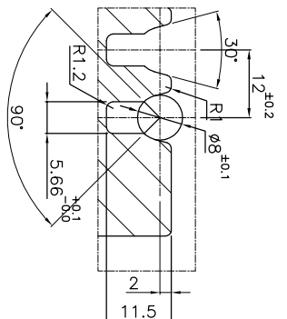
GROOVE DETAILS
